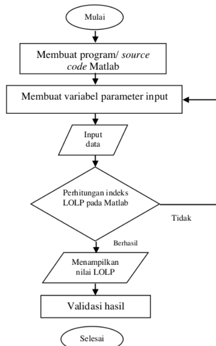
Gambar 1. Flowchart Penelitian
